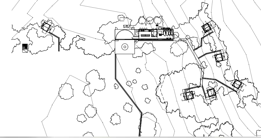
Site Plan (The Standing Camp – krakani lumi wukalina, Mt William National Park, Tasmania Architect: Taylor and Hinds Architects )
