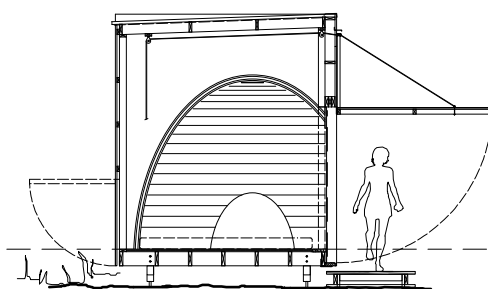
Elevation (The Standing Camp – krakani lumi wukalina, Mt William National Park, Tasmania Architect: Taylor and Hinds Architects)
